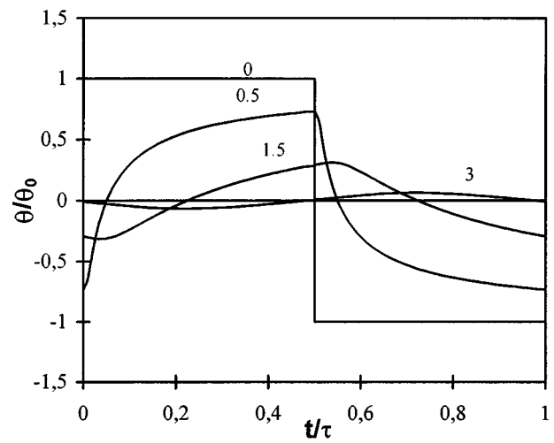
Fig. 1. Theoretical progressive harmonization of the wave at different distances from the sample origin.
