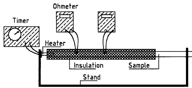
Fig. 2. Experimental setup.
