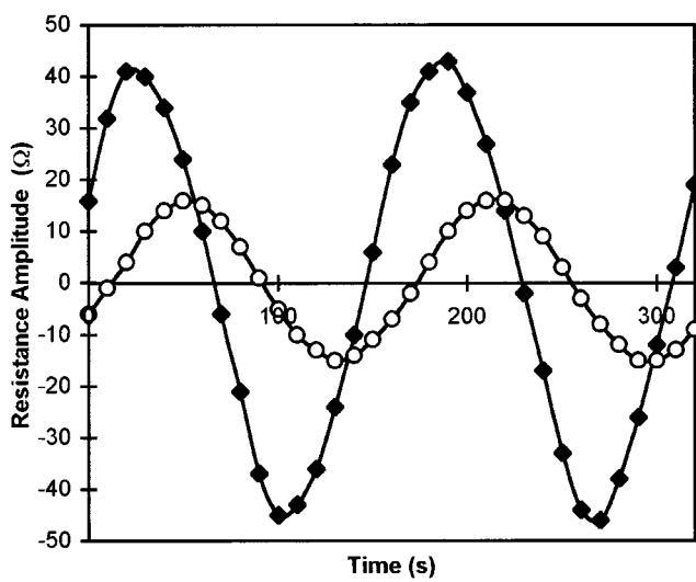
Fig. 4. Resistance amplitudes at 8 and 16 cm.
