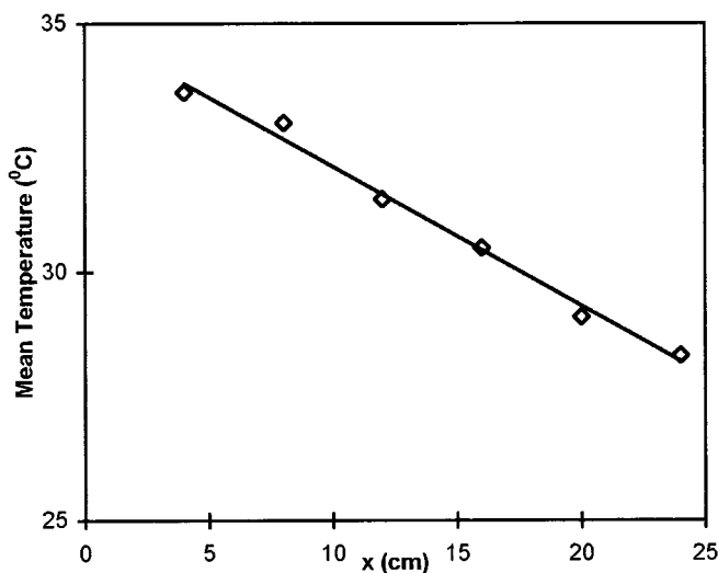
Fig. 5. Variation of the mean temperature along the bar.
